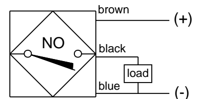
GPX-P (PNP) (Current sourcing)
