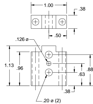
J1-1 jaw for B-1TPX (bolts & pins included)
